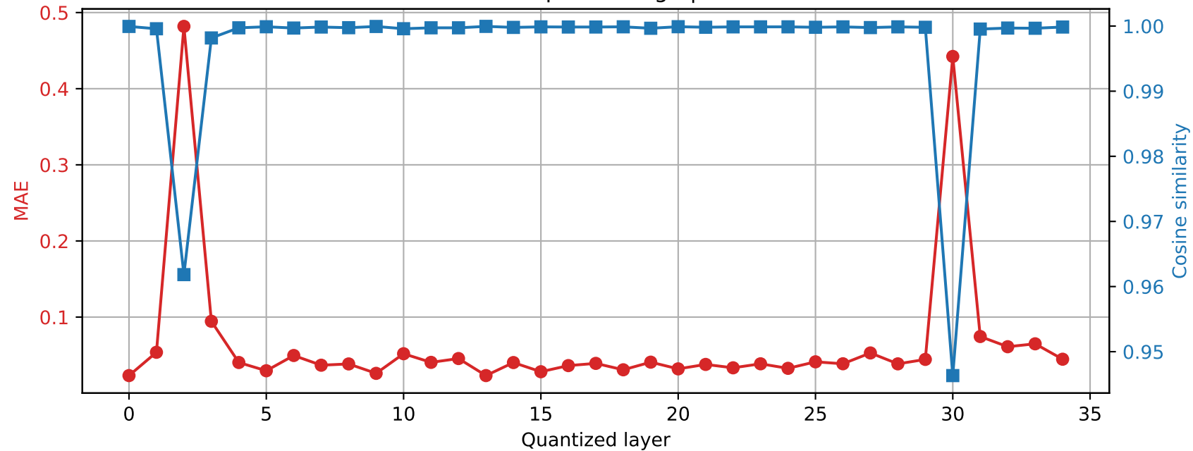
Qwen2.5-3B | Prompt 3 Final RMSNorm output damage | float64 → int8
