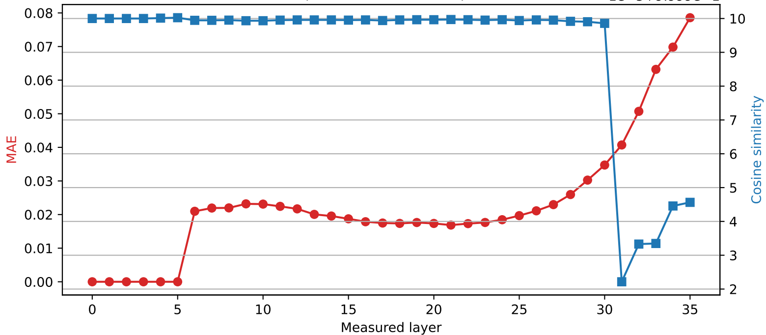
Qwen2.5-3B | Quantized layer 5 | float64 → int8
