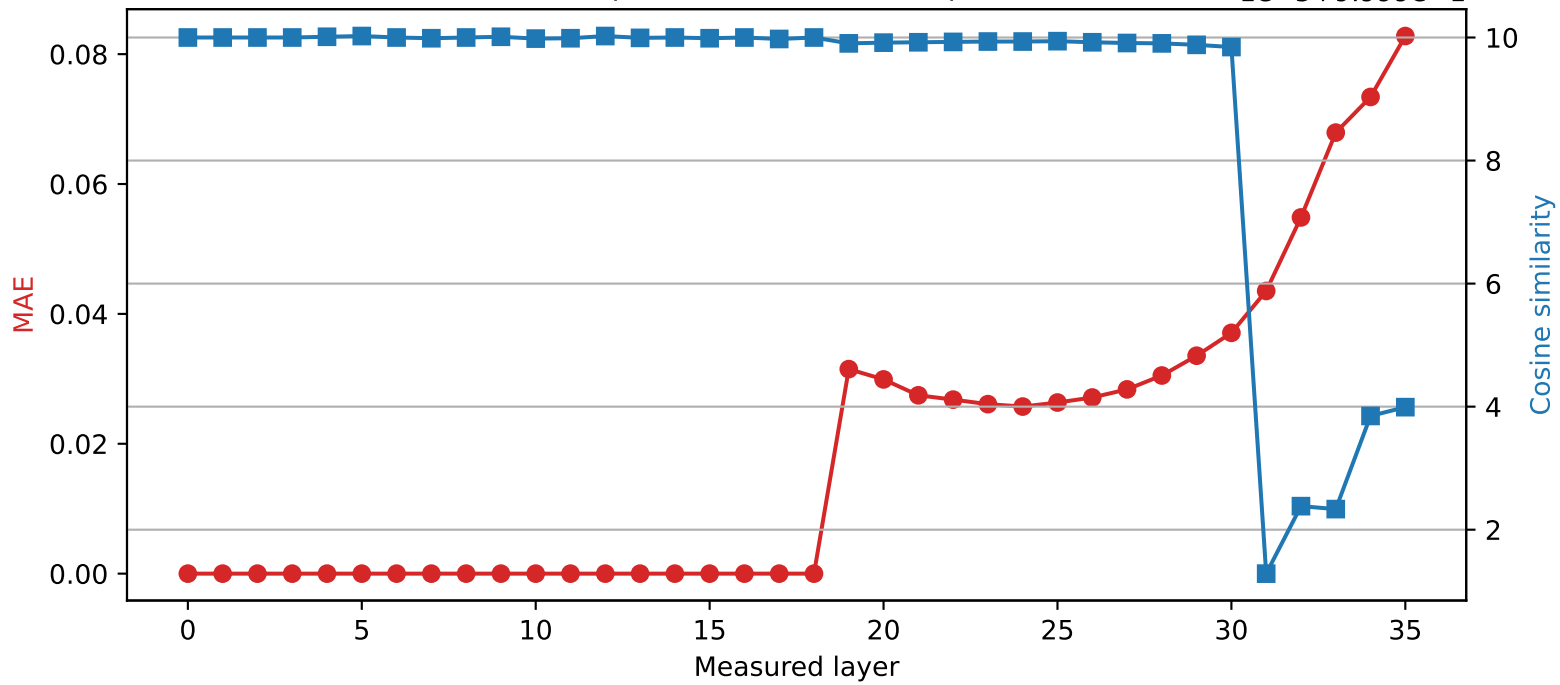
Qwen2.5-3B | Quantized layer 18 | float64 → int8
