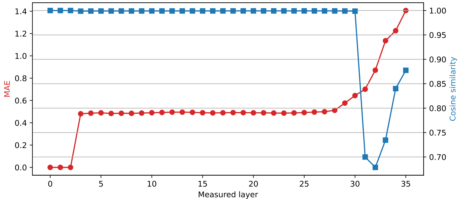
Qwen2.5-3B | Quantized layer 2 | float64 → int8
