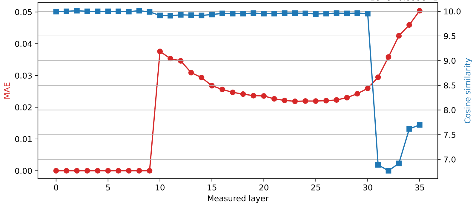
Qwen2.5-3B | Quantized layer 9 | float64 → int8
