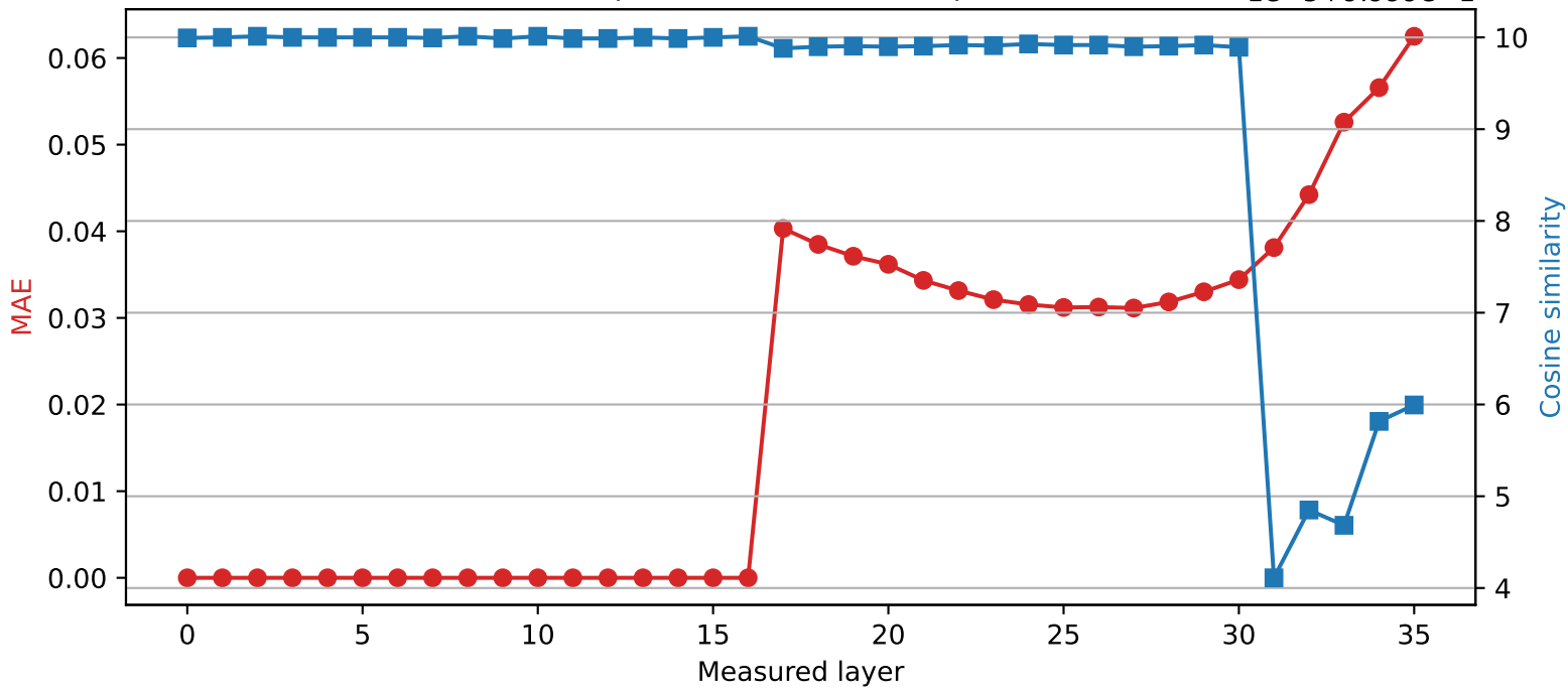
Qwen2.5-3B | Quantized layer 16 | float64 → int8
