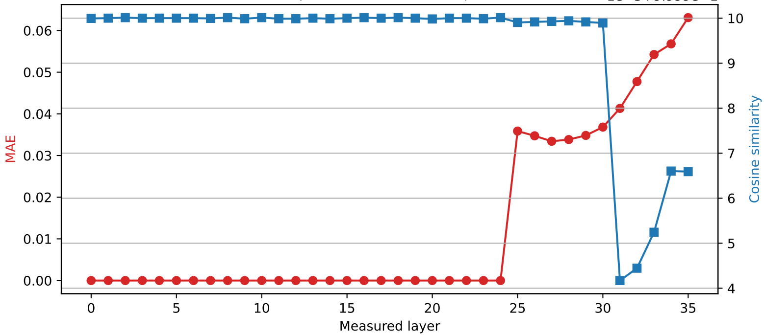
Qwen2.5-3B | Quantized layer 24 | float64 → int8
