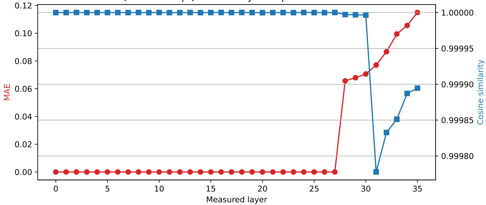
Qwen2.5-3B | Quantized layer 27 | float64 → int8
