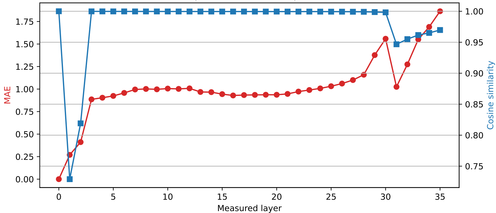
Qwen2.5-3B | Quantized layer 0 | float64 → int4
