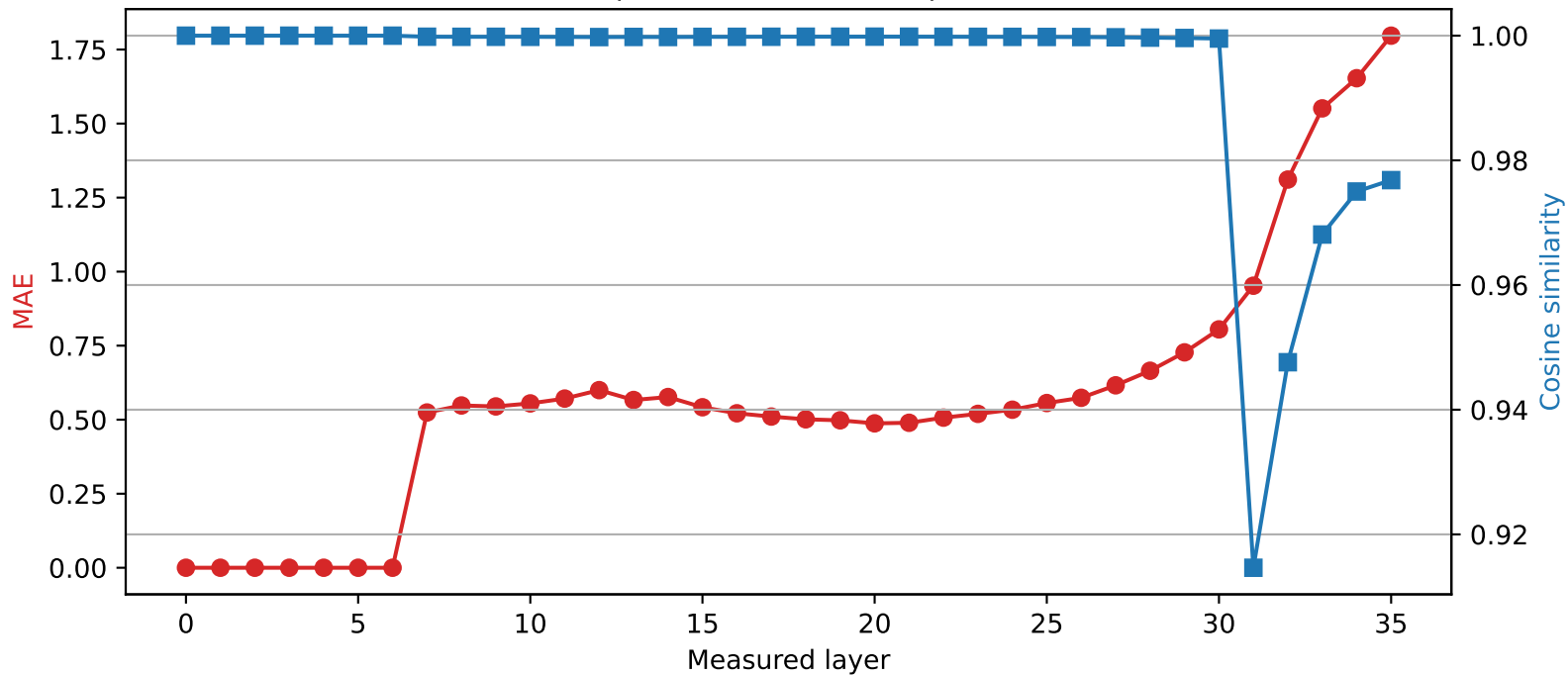
Qwen2.5-3B | Quantized layer 6 | float64 \rightarrow int4
