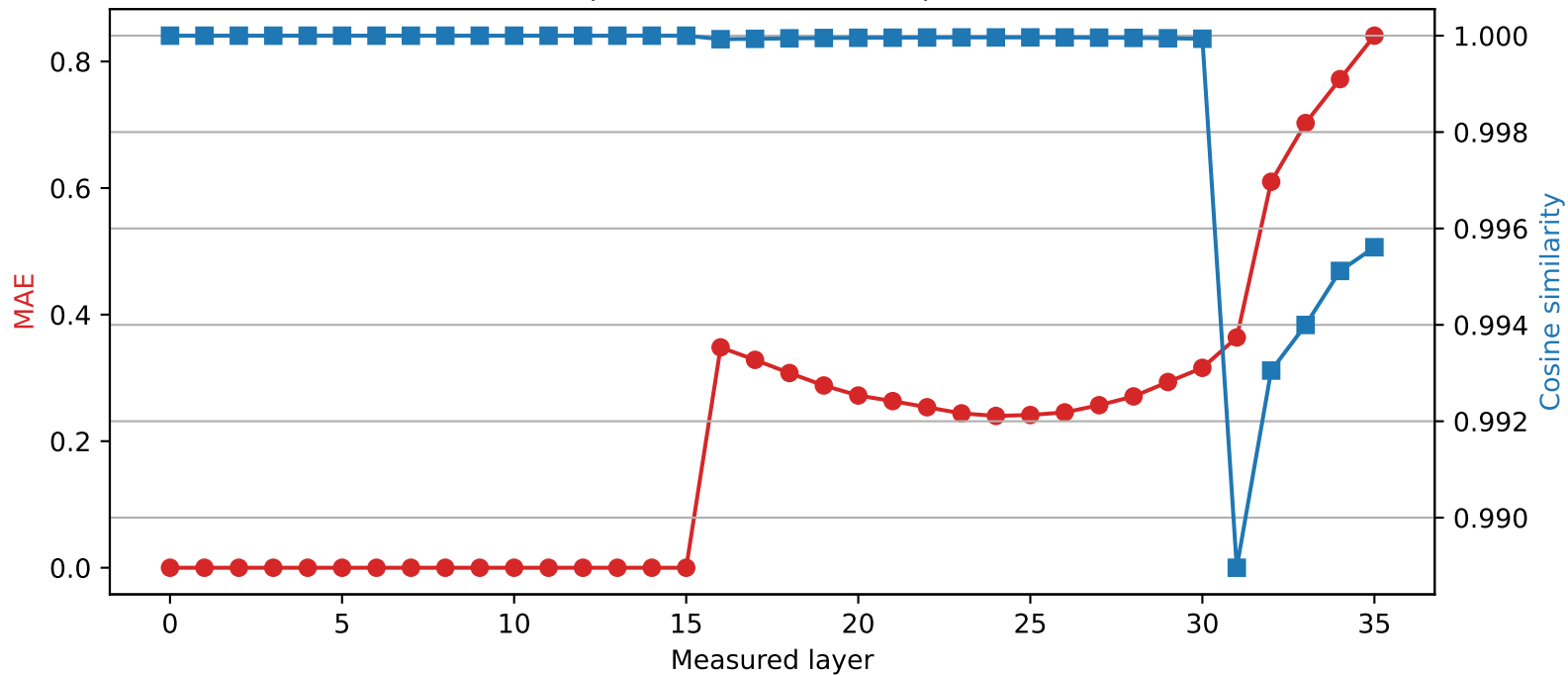
Qwen2.5-3B | Quantized layer 15 | float64 → int4
