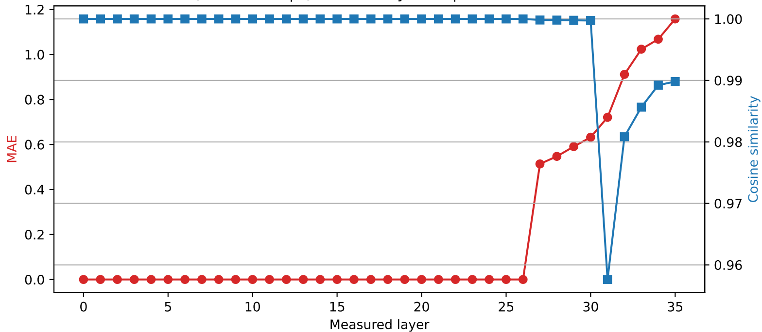
Qwen2.5-3B | Quantized layer 26 | float64 \rightarrow int4
