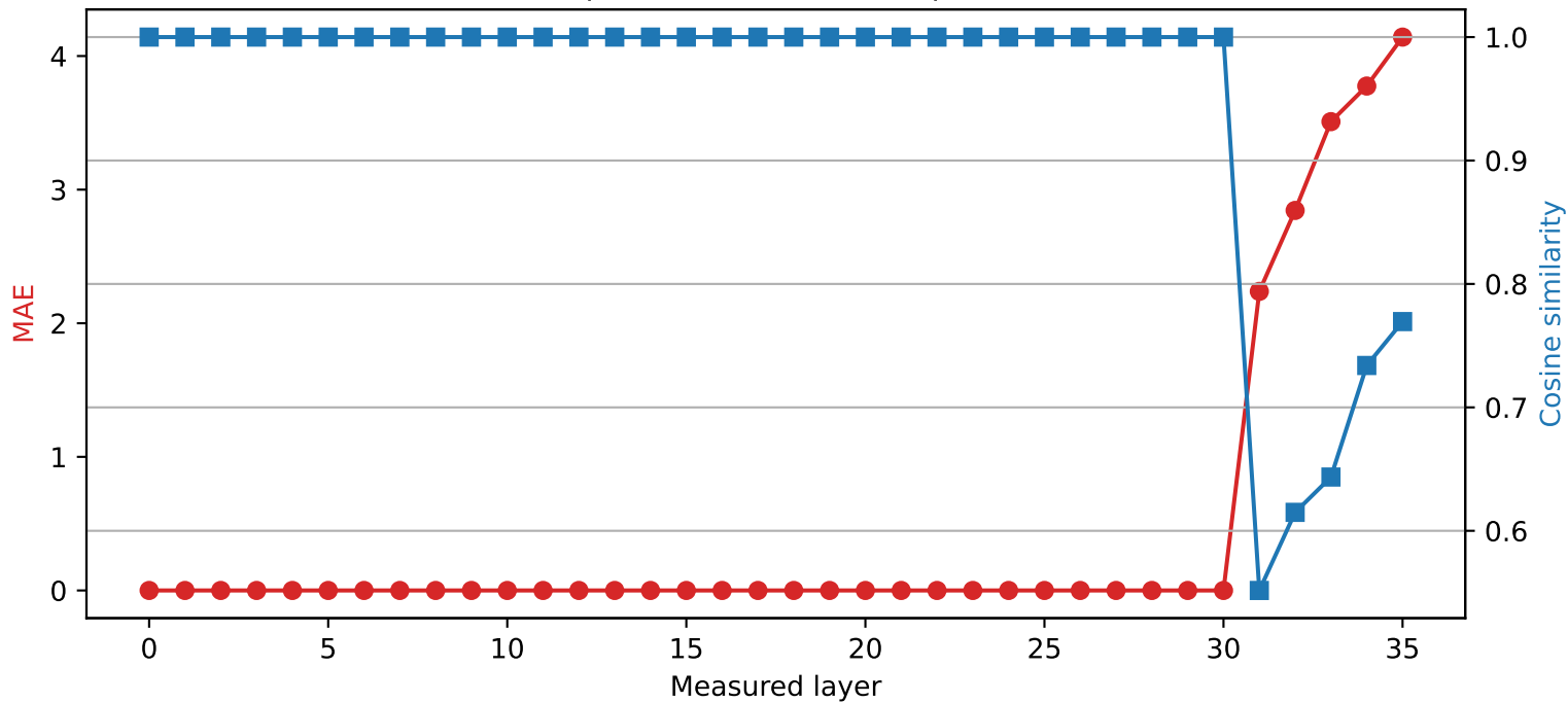
Qwen2.5-3B | Quantized layer 30 | float64 → int4
