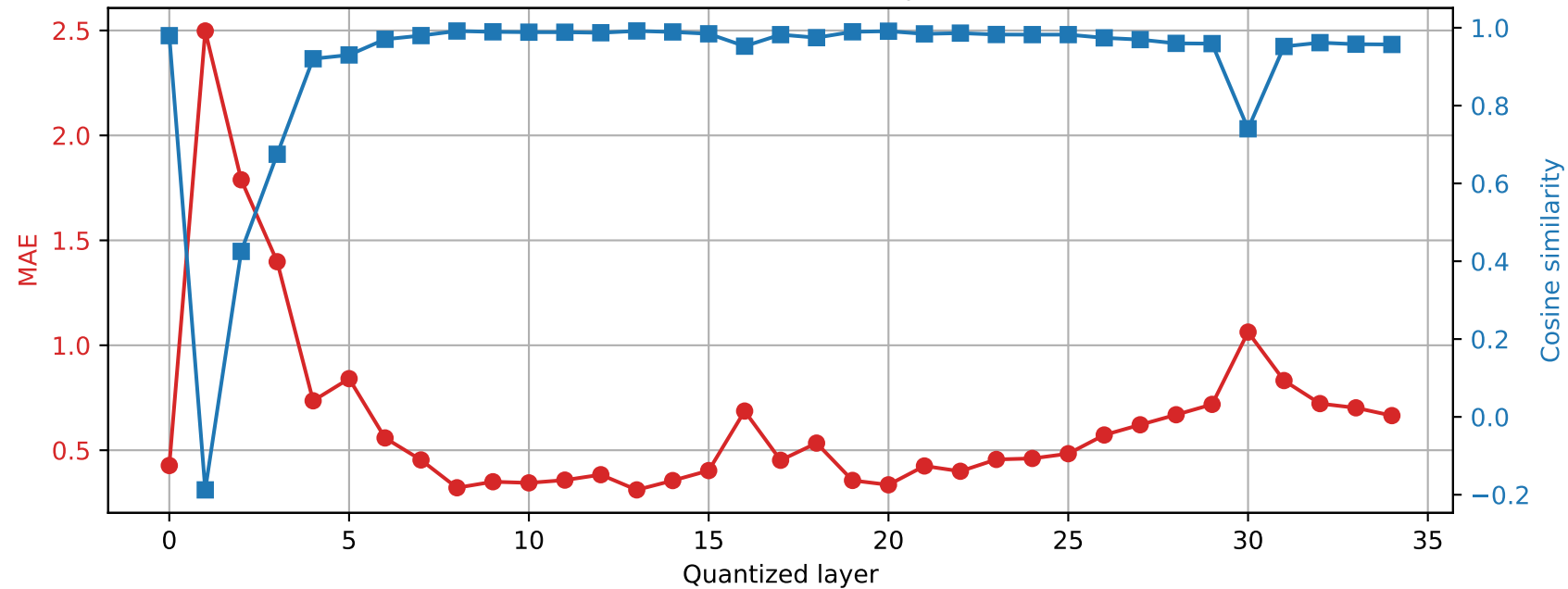
Qwen2.5-3B | Prompt 1 Final RMSNorm output damage | float64 \rightarrow int4
