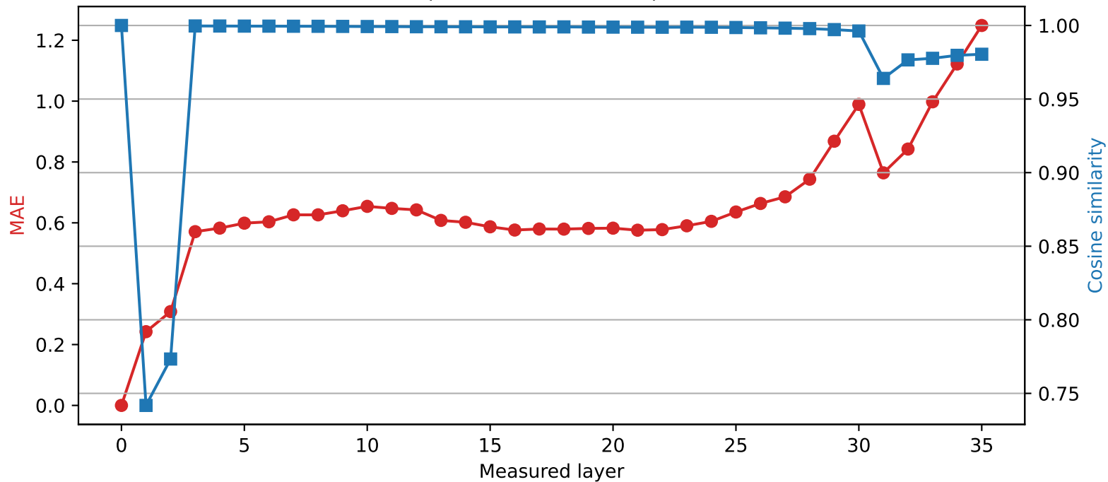
Qwen2.5-3B | Quantized layer 0 | float64 \rightarrow int4
