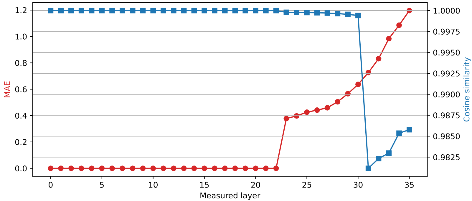
Qwen2.5-3B | Quantized layer 22 | float64 → int4
