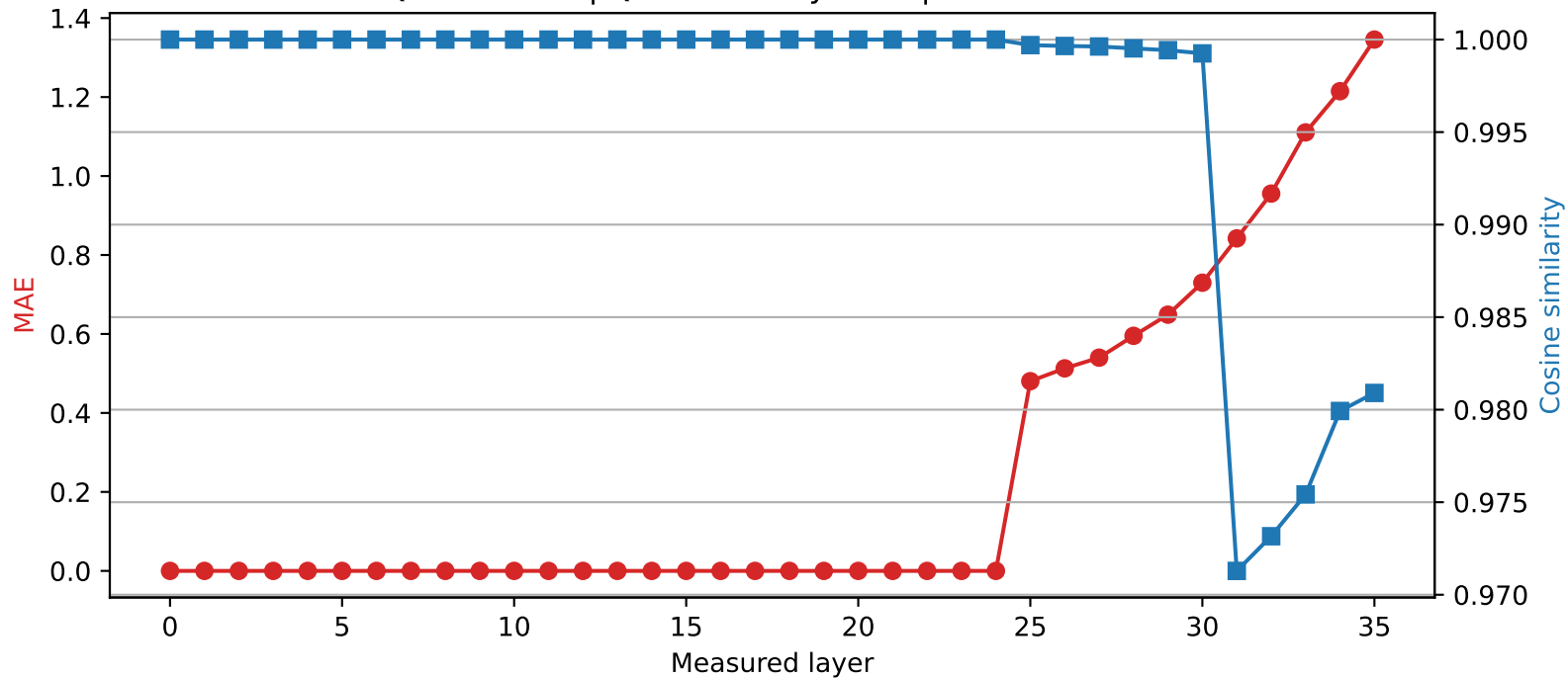
Qwen2.5-3B | Quantized layer 24 | float64 → int4
