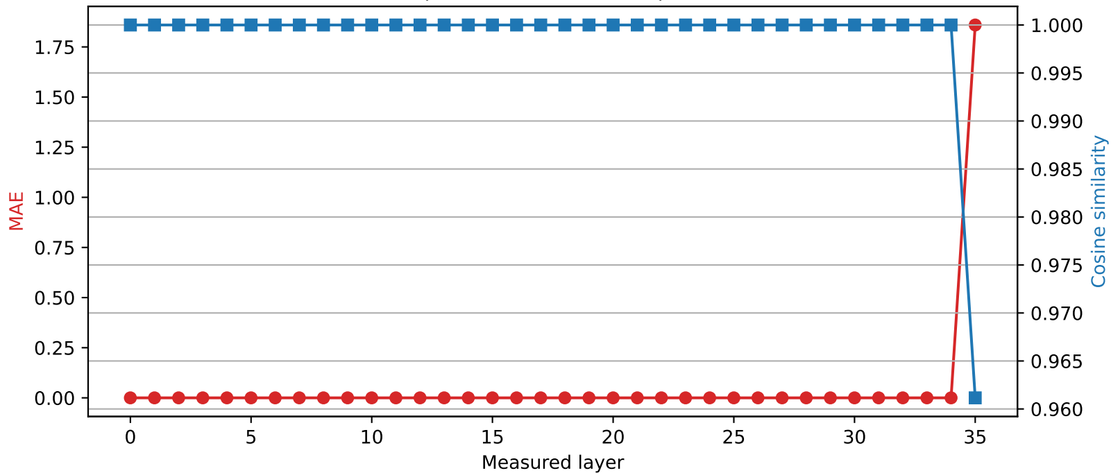
Qwen2.5-3B | Quantized layer 34 | float64 → int4
