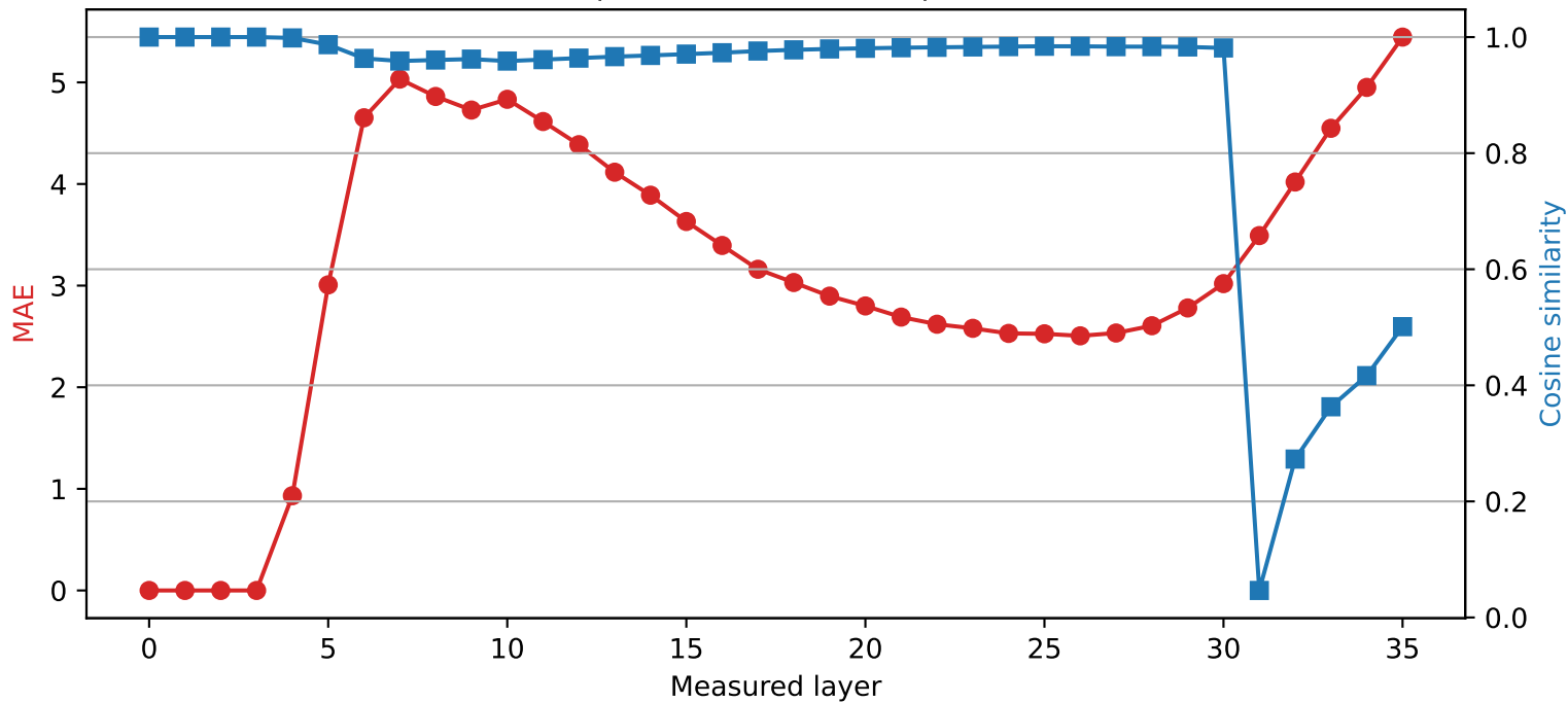
Qwen2.5-3B | Quantized layer 3 | float64 → int4
