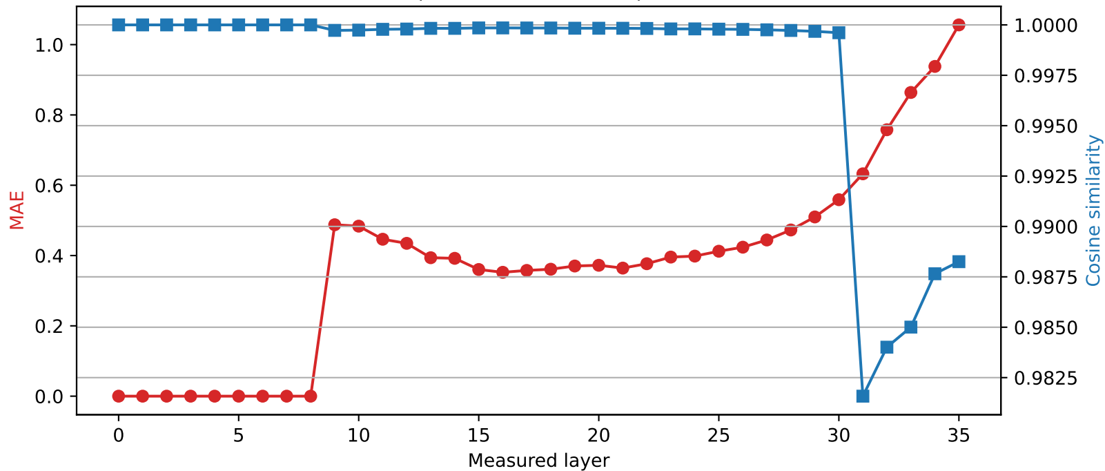
Qwen2.5-3B | Quantized layer 8 | float64 → int4
