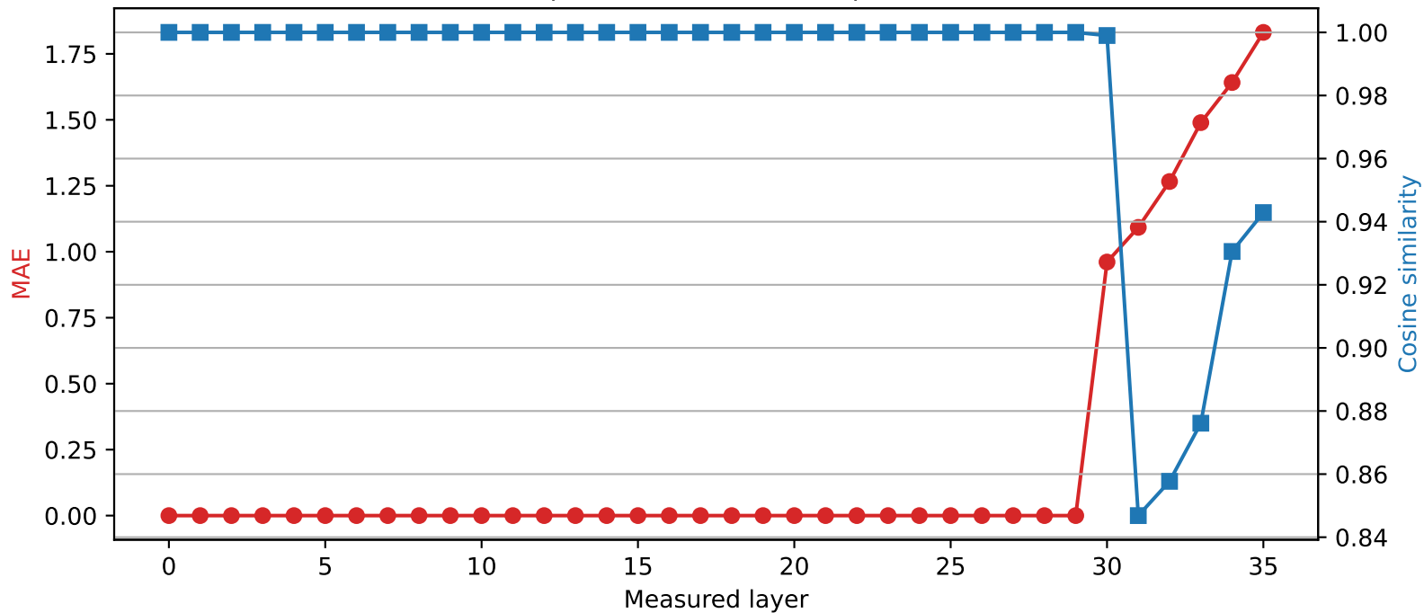
Qwen2.5-3B | Quantized layer 29 | float64 \rightarrow int4
