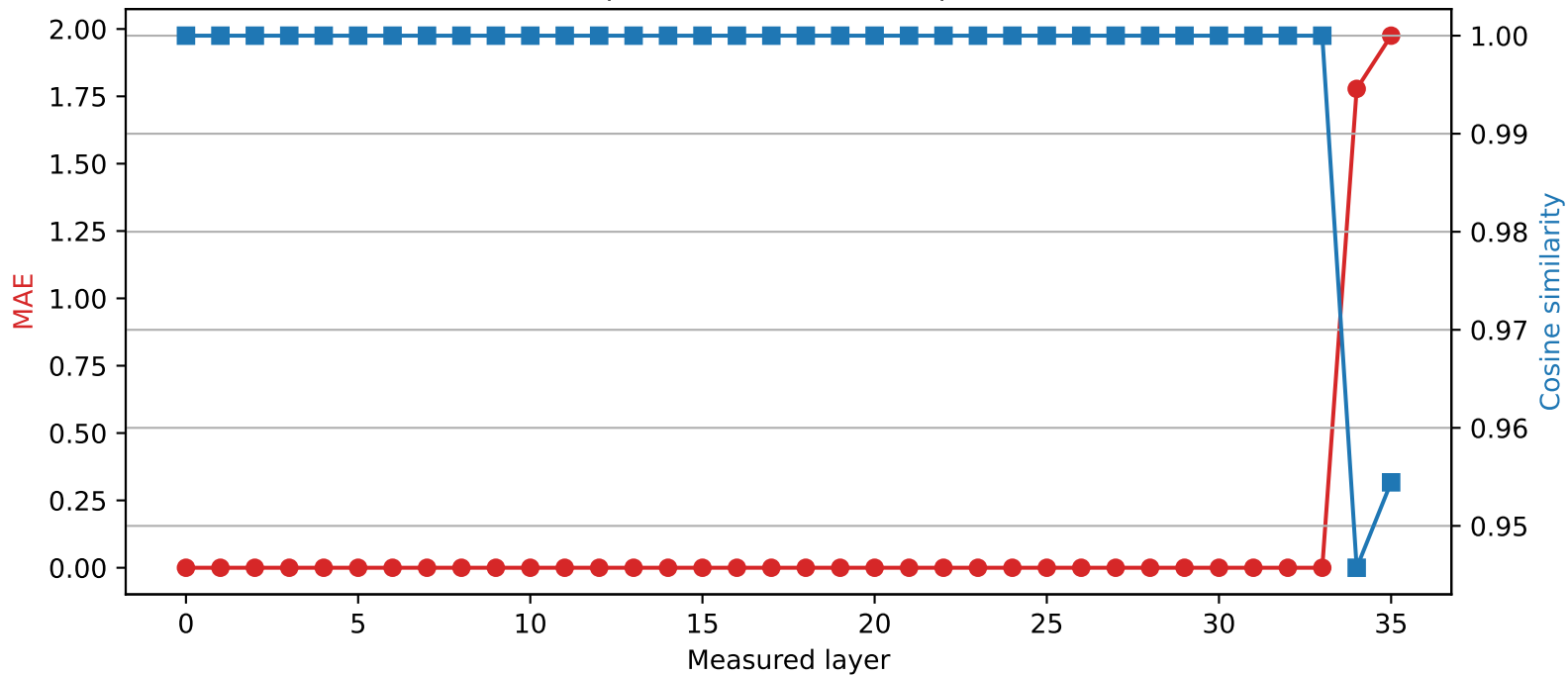
Qwen2.5-3B | Quantized layer 33 | float64 \rightarrow int4
