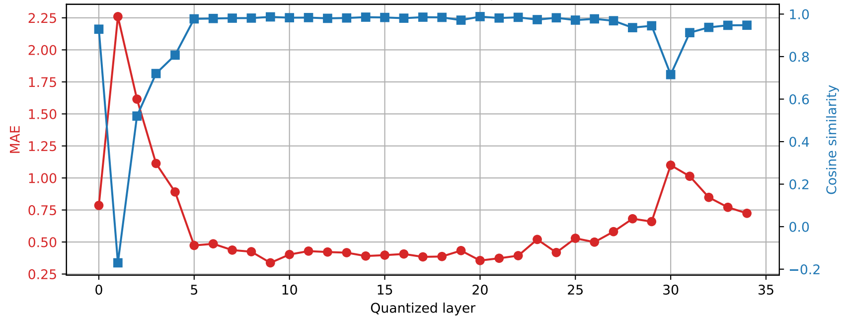
Qwen2.5-3B | Prompt 3 Final RMSNorm output damage | float64 \rightarrow int4
