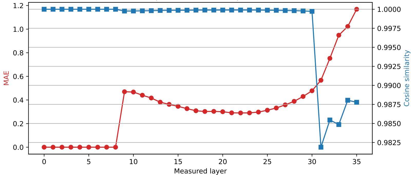
Qwen2.5-3B | Quantized layer 8 | float64 \rightarrow int4
