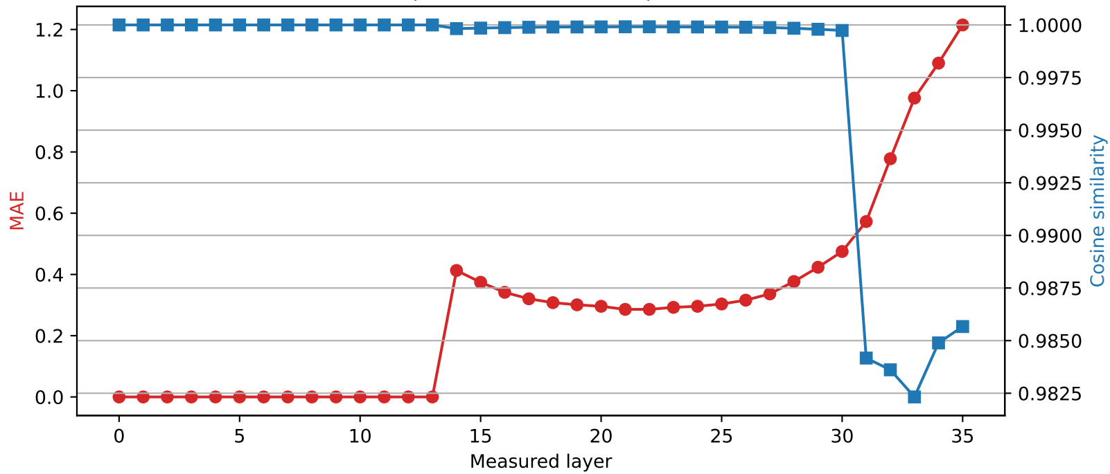
Qwen2.5-3B | Quantized layer 13 | float64 → int4
