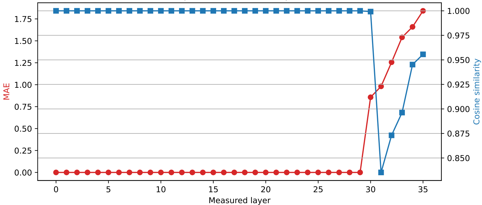
Qwen2.5-3B | Quantized layer 29 | float64 → int4
