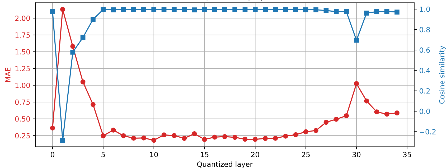
Qwen2.5-3B | Prompt 4 Final RMSNorm output damage | float64 \rightarrow int4
