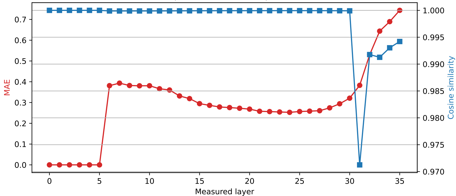
Qwen2.5-3B | Quantized layer 5 | float64 \rightarrow int4
