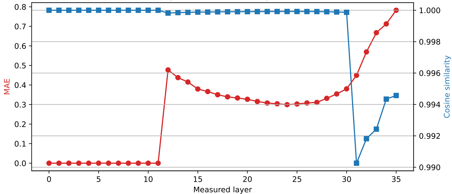
Qwen2.5-3B | Quantized layer 11 | float64 → int4
