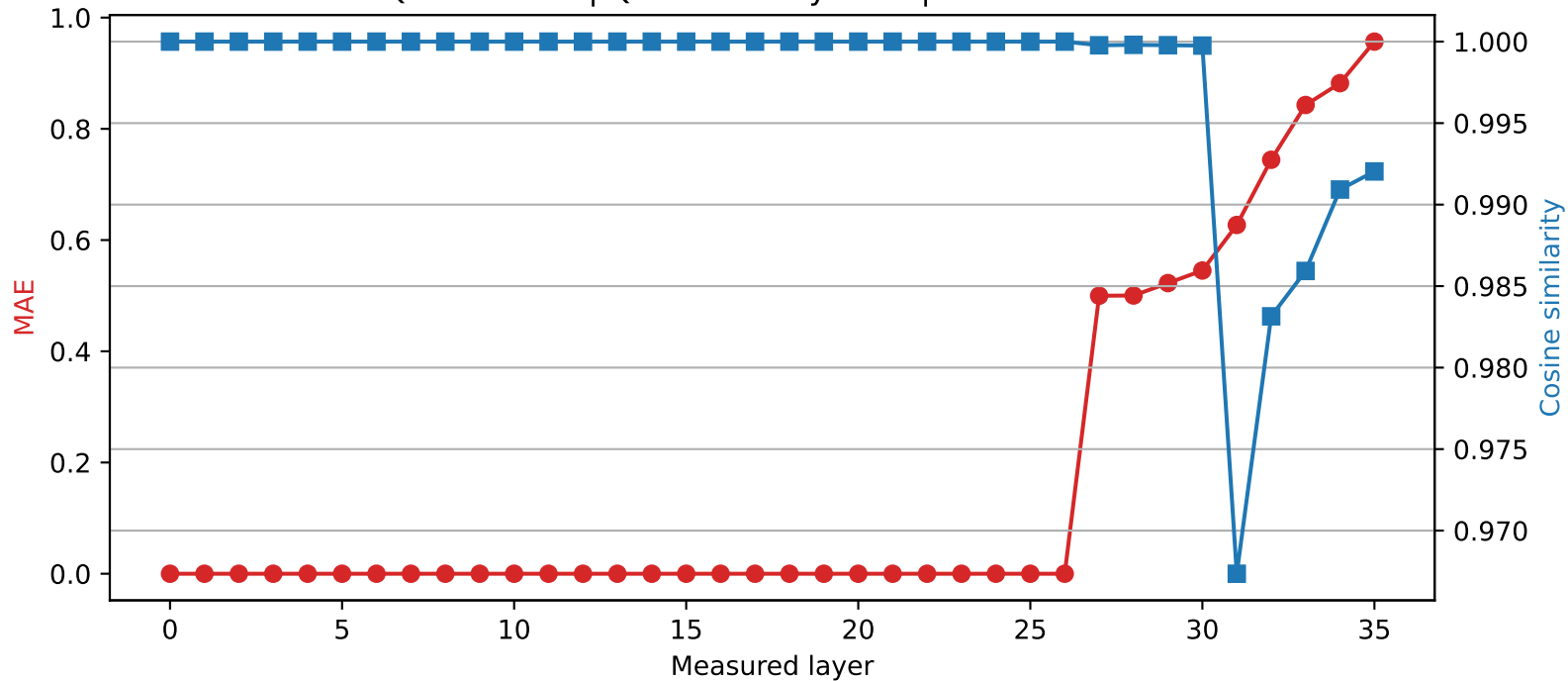
Qwen2.5-3B | Quantized layer 26 | float64 → int4
