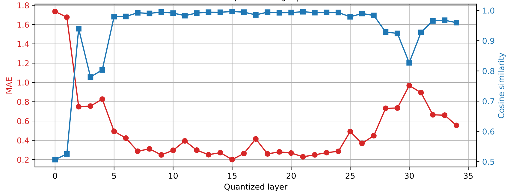
Qwen2.5-3B | Prompt 0 Final RMSNorm output damage | float64 \rightarrow int2
