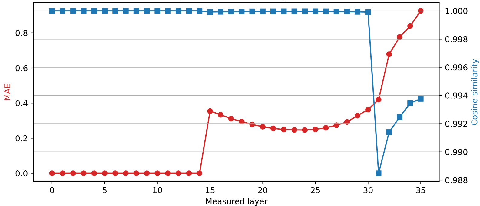
Qwen2.5-3B | Quantized layer 14 | float64 → int2
