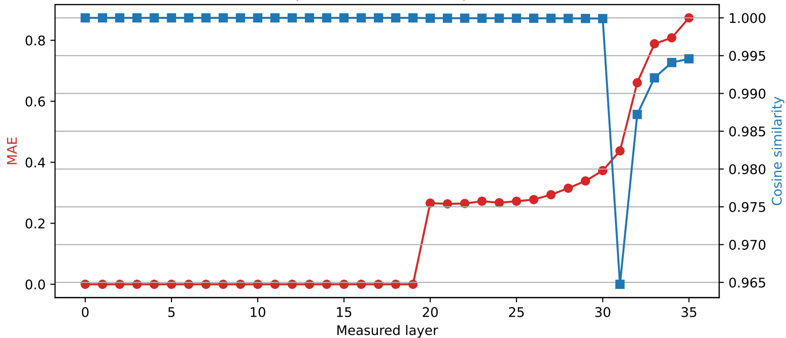
Qwen2.5-3B | Quantized layer 19 | float64 → int2
