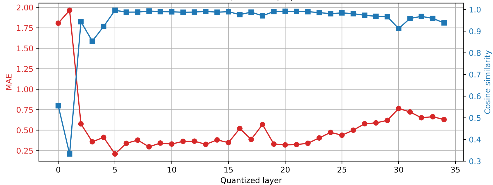
Qwen2.5-3B | Prompt 1 Final RMSNorm output damage | float64 → int2
