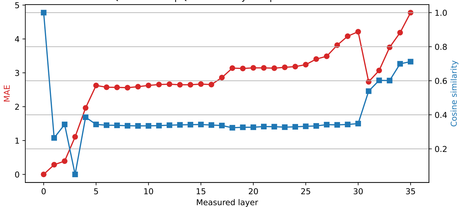
Qwen2.5-3B | Quantized layer 0 | float64 → int2
