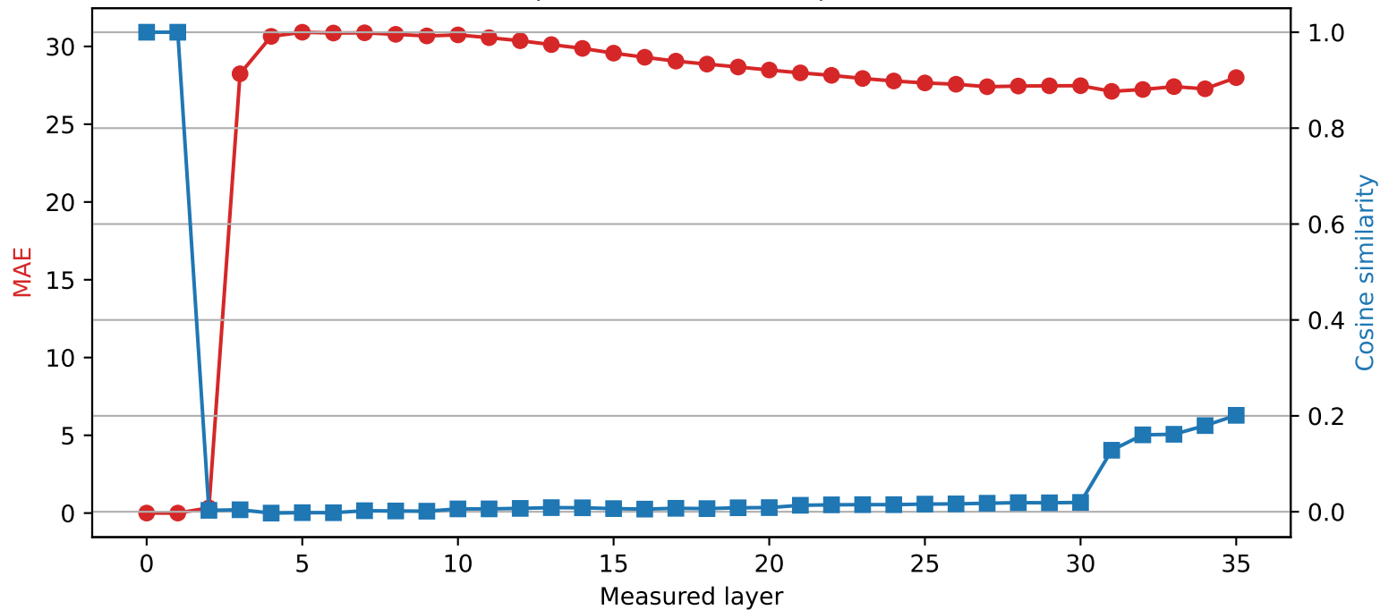
Qwen2.5-3B | Quantized layer 1 | float64 \rightarrow int2
