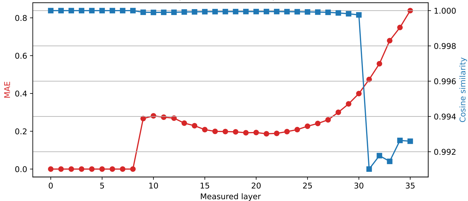
Qwen2.5-3B | Quantized layer 8 | float64 \rightarrow int2
