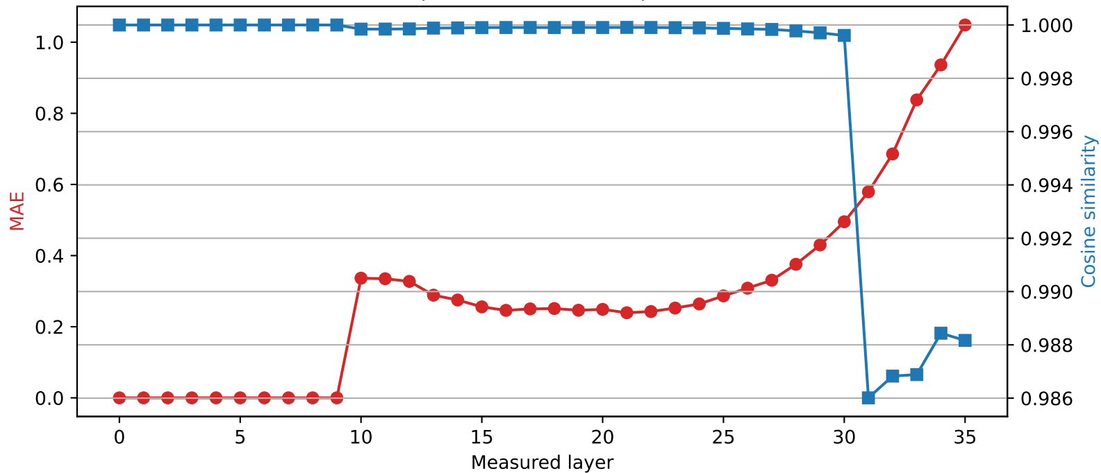
Qwen2.5-3B | Quantized layer 9 | float64 \rightarrow int2
