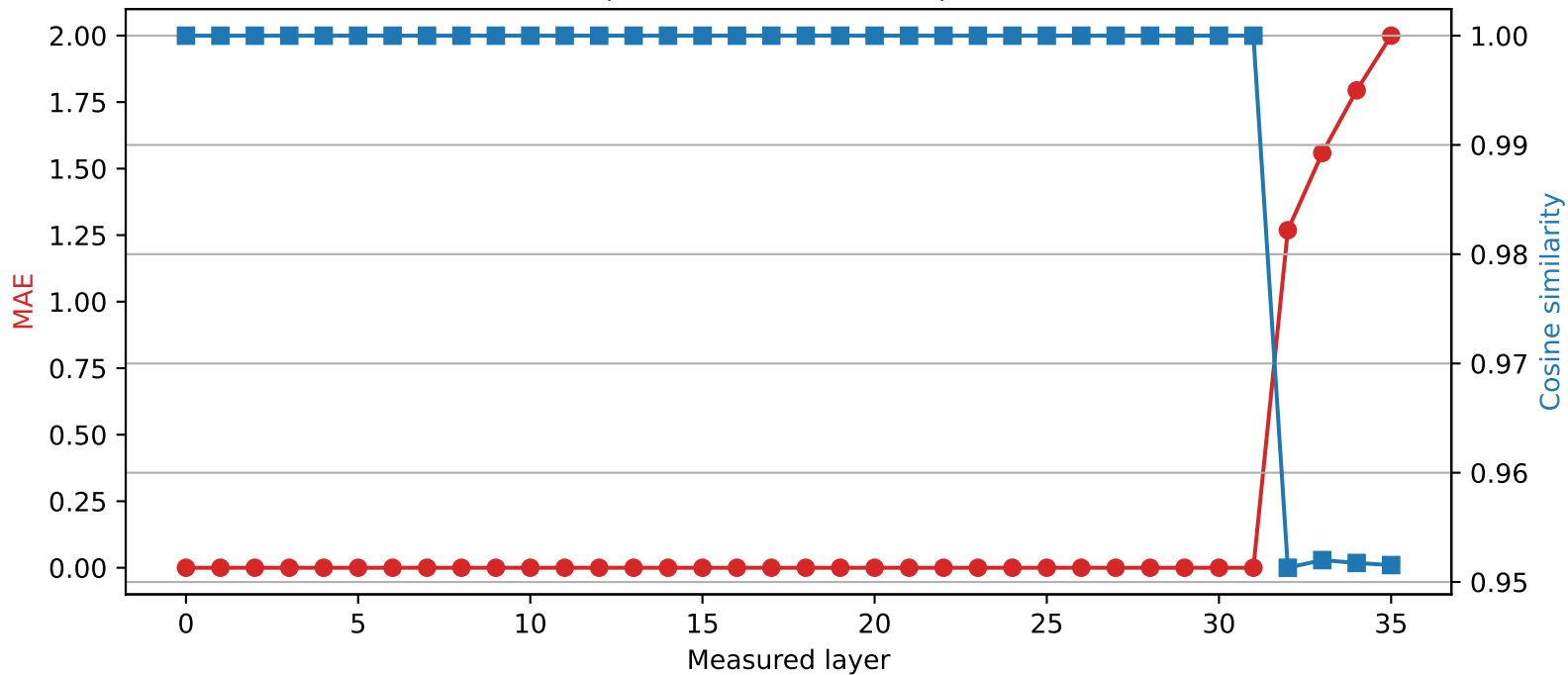
Qwen2.5-3B | Quantized layer 31 | float64 \rightarrow int2
