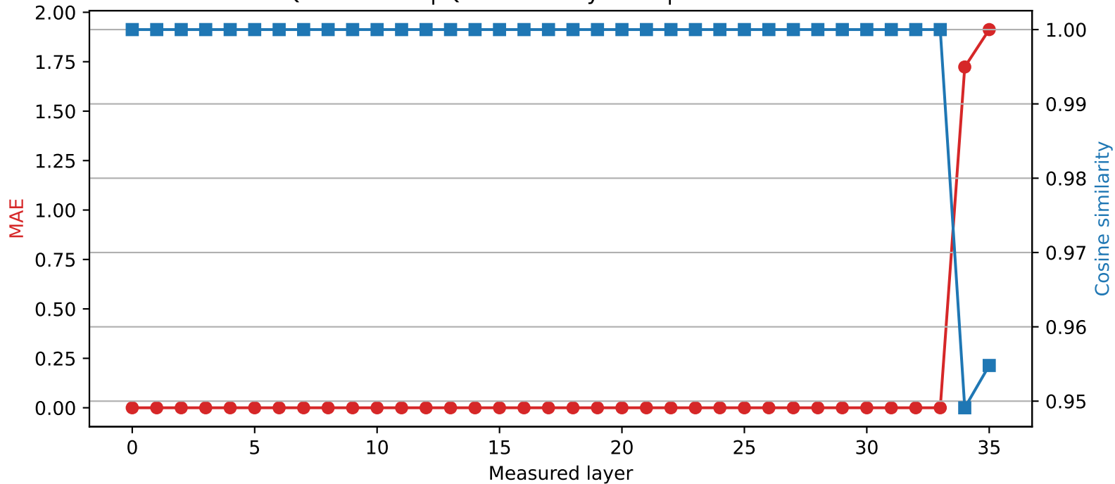
Qwen2.5-3B | Quantized layer 33 | float64 \rightarrow int2
