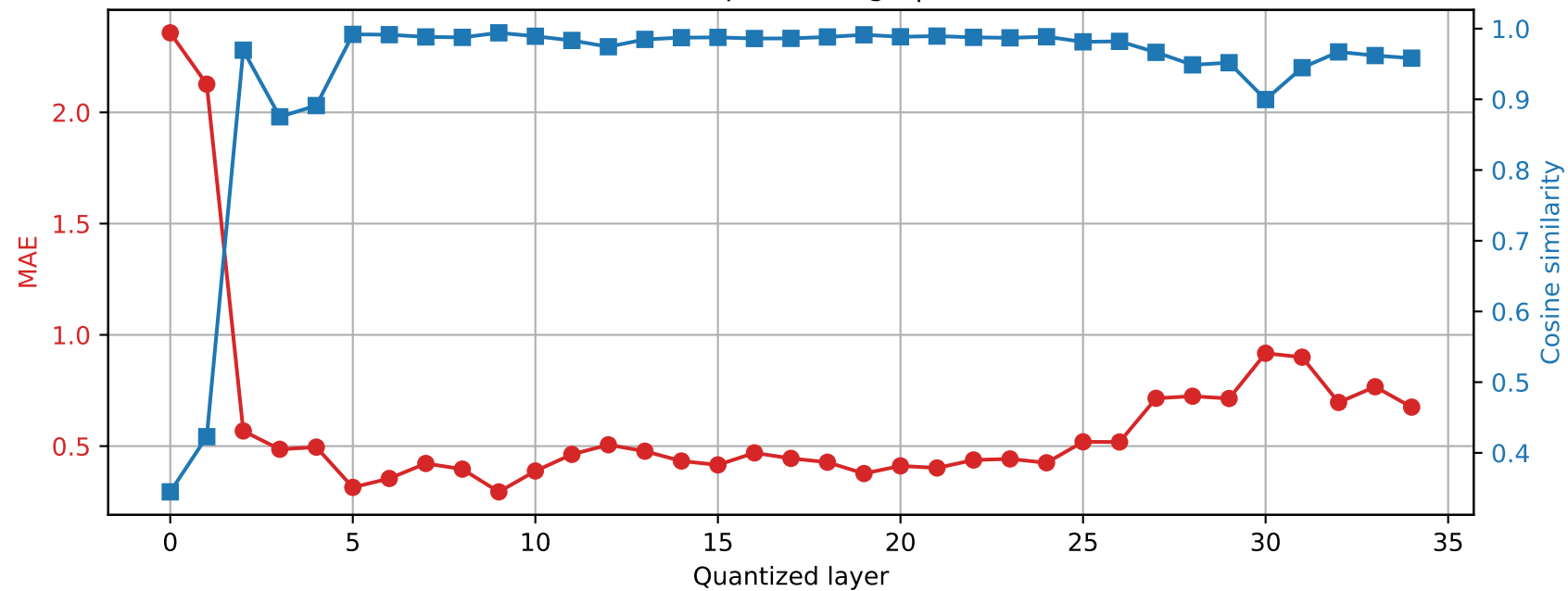
Qwen2.5-3B | Prompt 2 Final RMSNorm output damage | float64 \rightarrow int2
