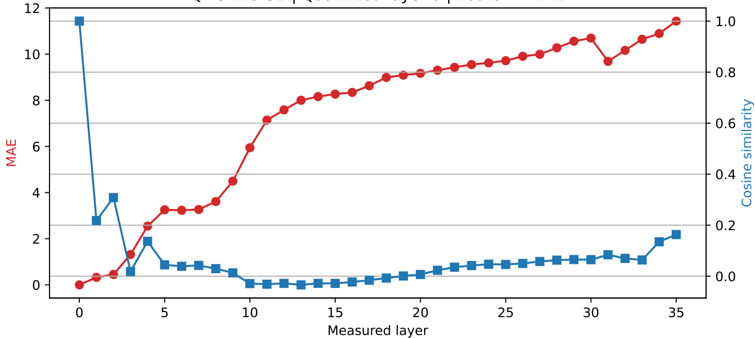
Qwen2.5-3B | Quantized layer 0 | float64 \rightarrow int2
