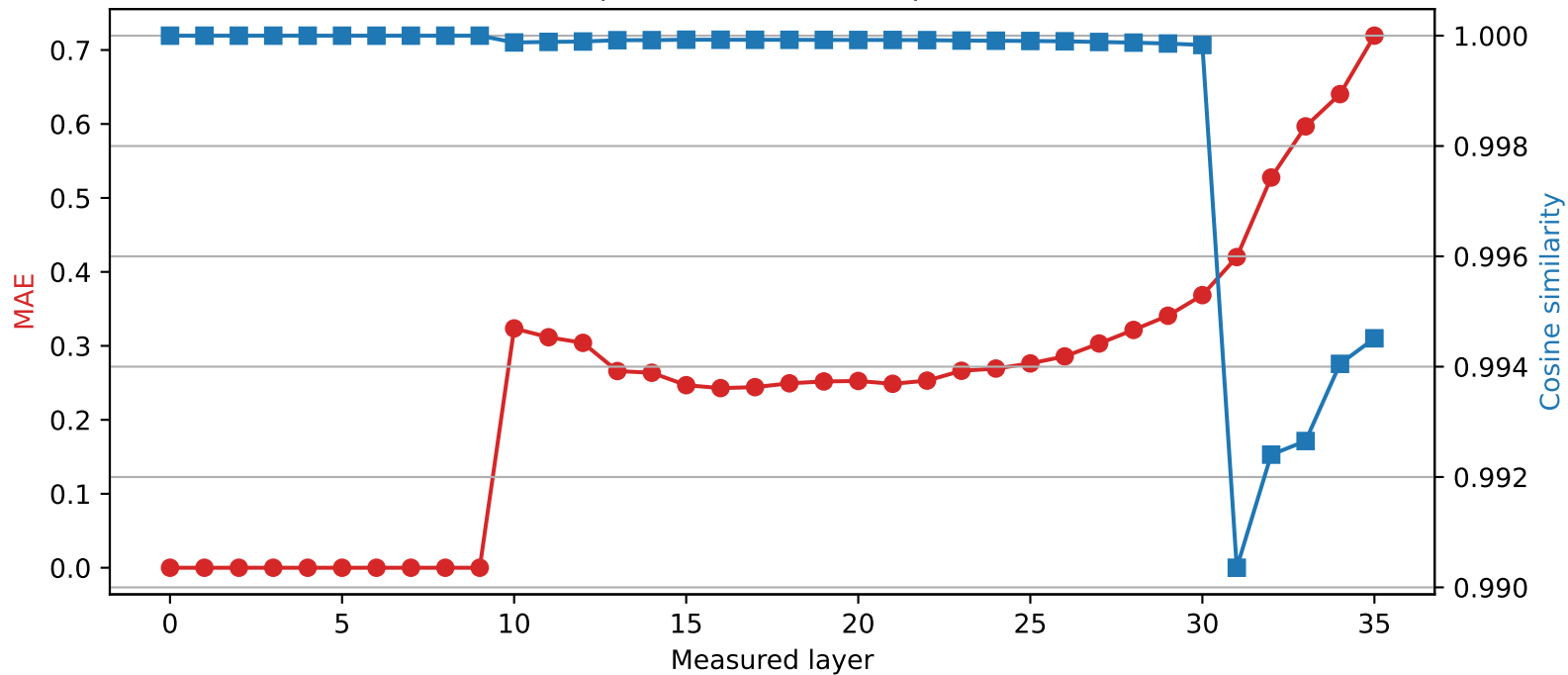
Qwen2.5-3B | Quantized layer 9 | float64 → int2
