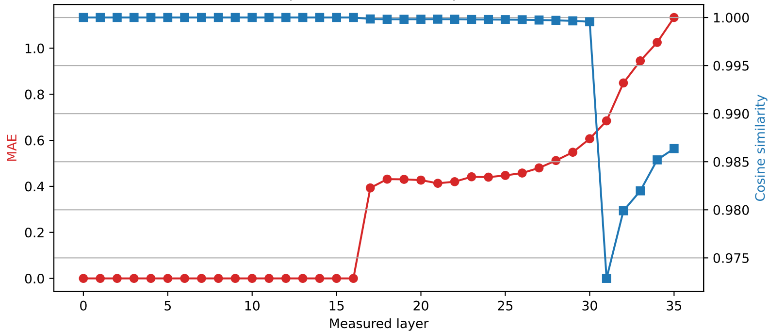
Qwen2.5-3B | Quantized layer 16 | float64 → int2
