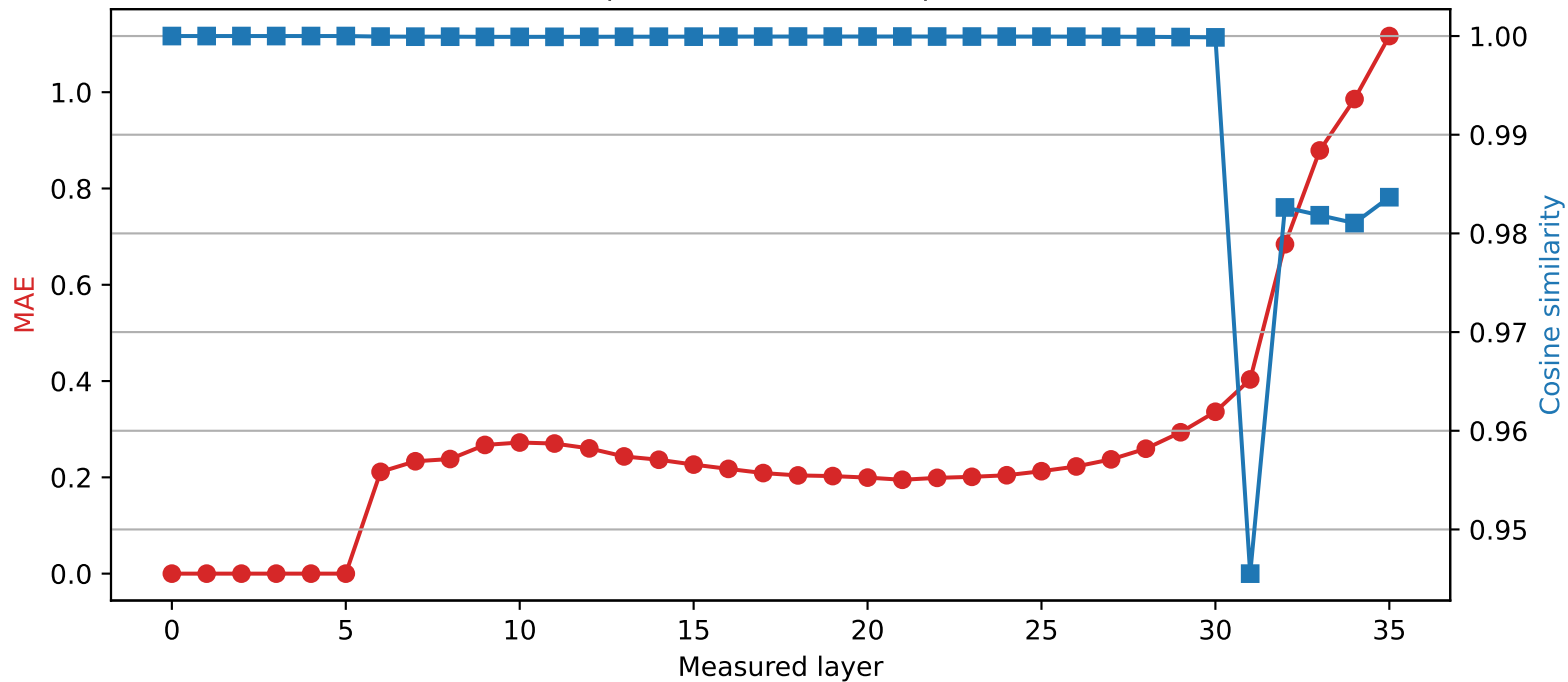
Qwen2.5-3B | Quantized layer 5 | float64 \rightarrow int2
