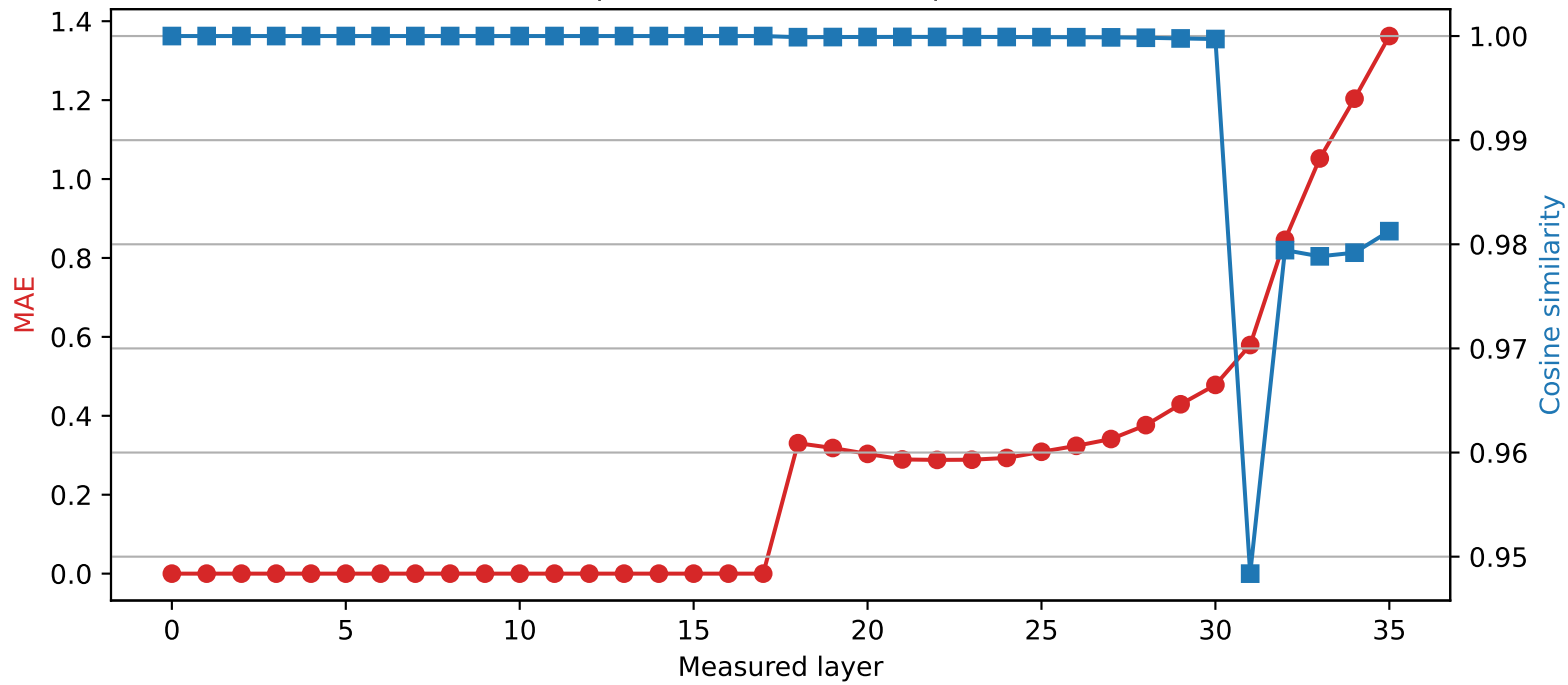
Qwen2.5-3B | Quantized layer 17 | float64 → int2
