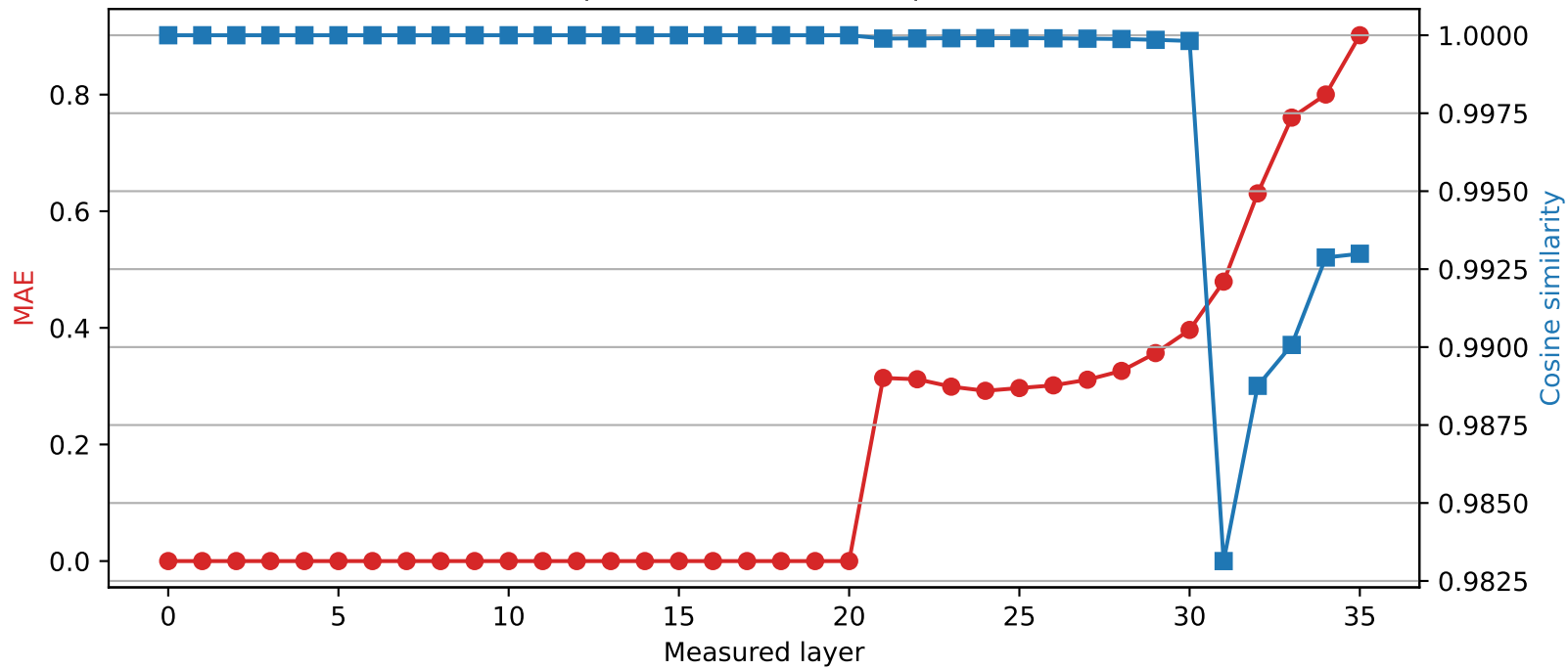
Qwen2.5-3B | Quantized layer 20 | float64 → int2
