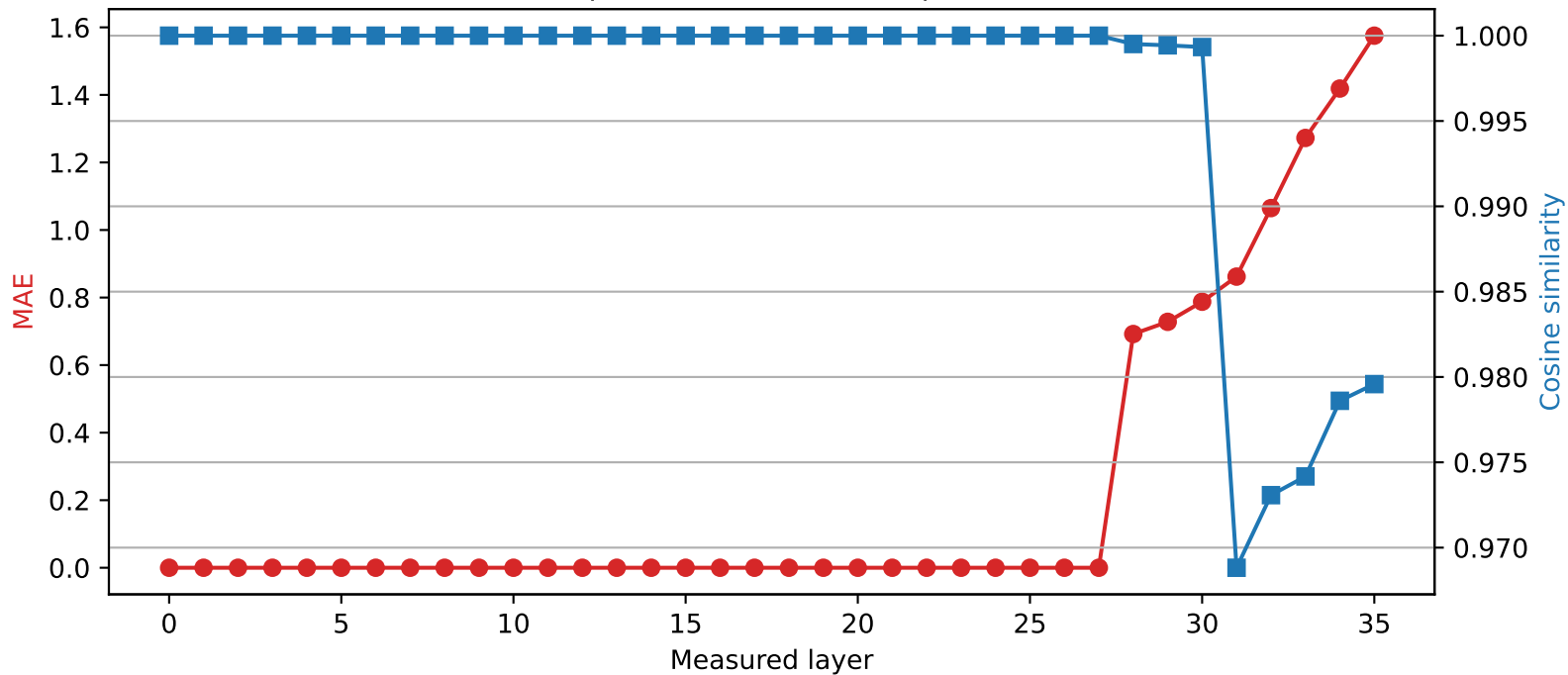
Qwen2.5-3B | Quantized layer 27 | float64 → int2
