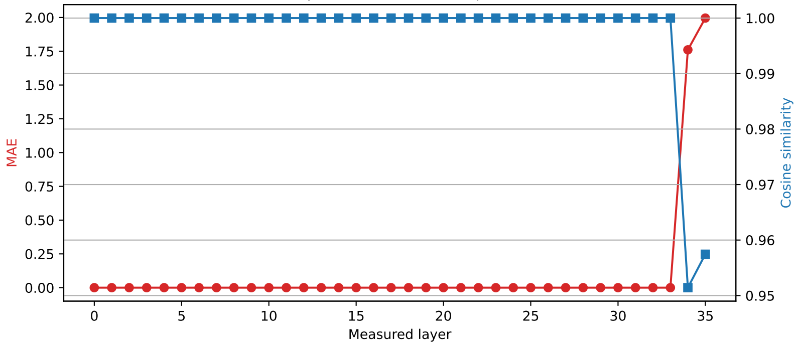
Qwen2.5-3B | Quantized layer 33 | float64 → int2
