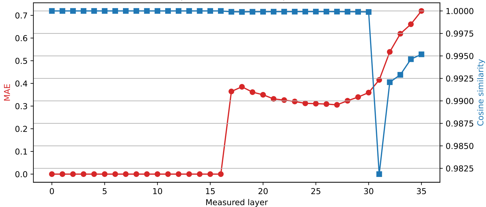
Qwen2.5-3B | Quantized layer 16 | float64 \rightarrow int2
